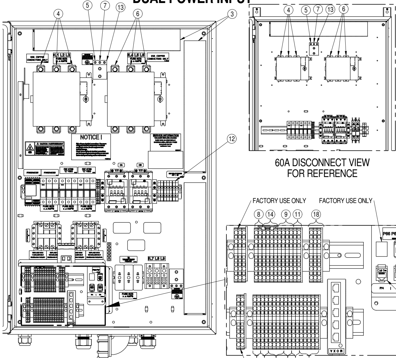
200A DISCONNECT VIEW
