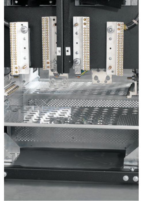
Ground and neutral output connections are conveniently located in the bottom of the unit for easy wiring. Conduit-landing plate provided with plugged holes — no knock-outs.
