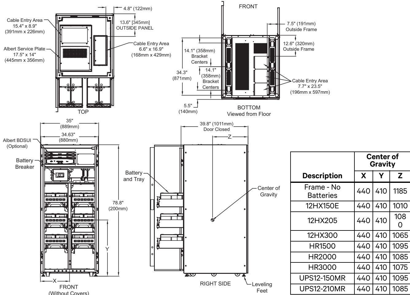
Figure 13 Battery cabinet outline drawing and main components—880mm cabinet
