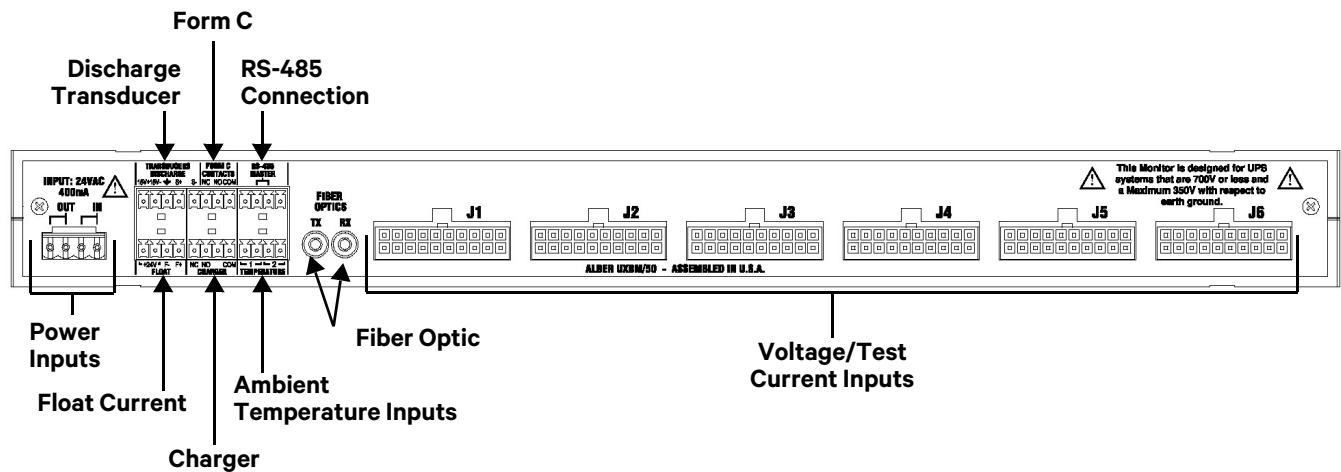
Figure 11 Alber BDSUi-UXBM/50 rear panel
