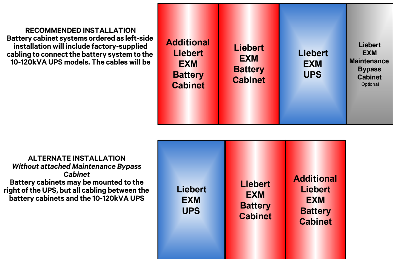
Figure 1 Battery cabinets connected, attached to UPS
