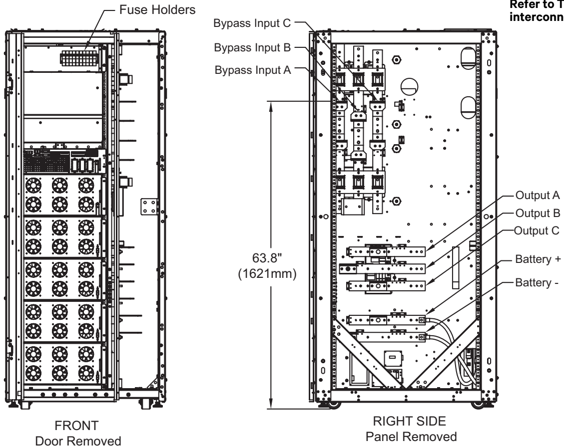
Figure 7 Liebert EXM UPS terminal detail 250kVA
