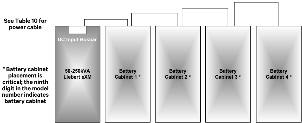
Figure 3 Power cabling for 50-250kVA UPS
