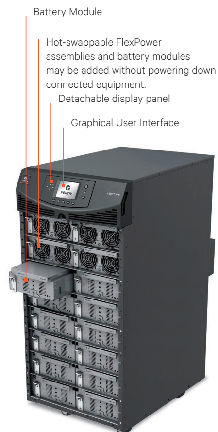
Fully populated Liebert APS complete with both power and battery modules.
