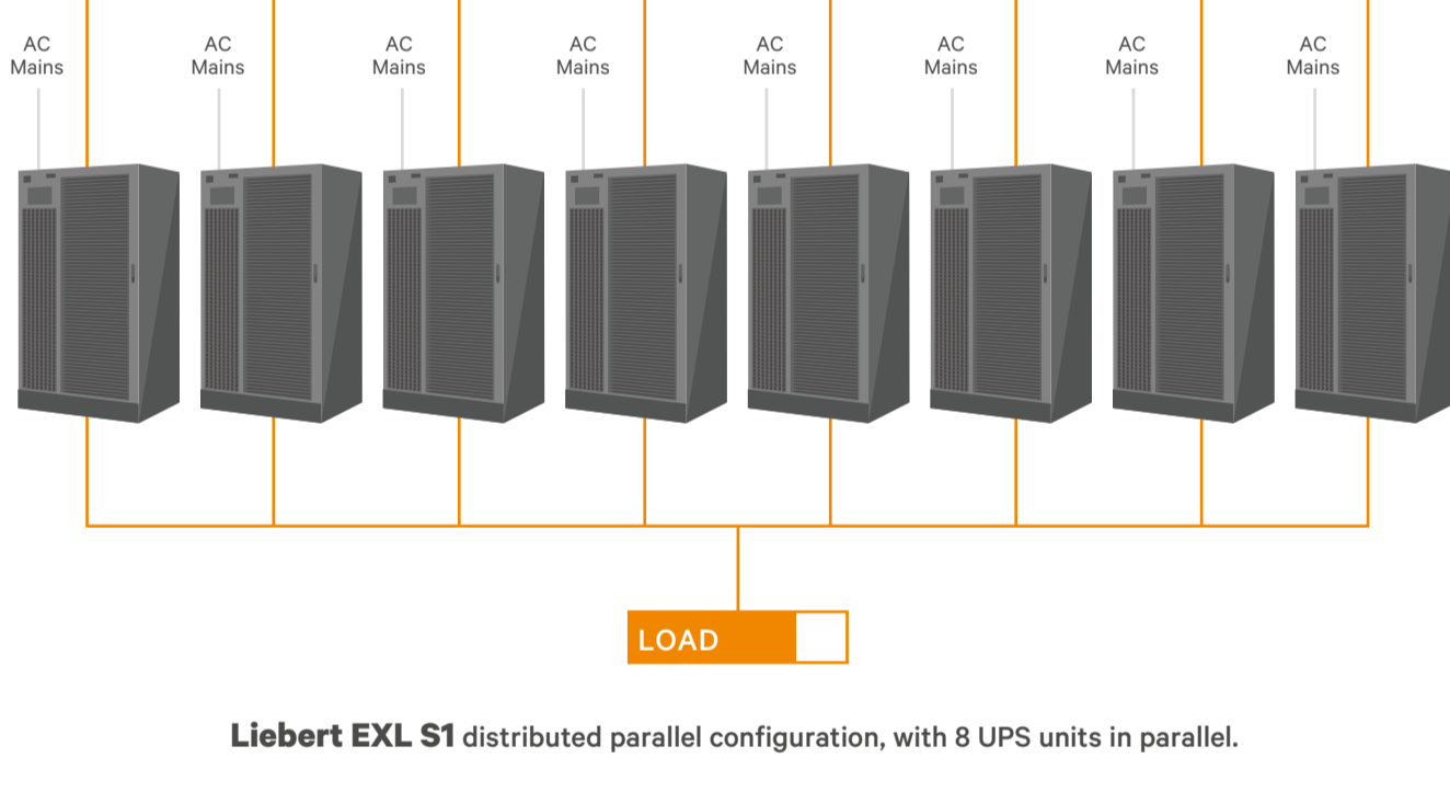
Liebert EXL S1 distributed parallel configuration, with 8 UPS units in parallel.
